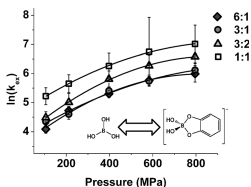
Figure 3. \ln(k_{\text{ex}}) as a function of pressure for various H 3 BO 3 (0.3 M) / catechol solution compositions at T = 323 K. The data are fitted to the quadratic Equation (3) with the resulting apparent activation parameters compiled in Table 1. The inset shows the two 11 B species used to calculate k ex from the 11 B NMR spectra acquired on the high-pressure cell NMR probe. The error bars indicate the standard error of each datum.
